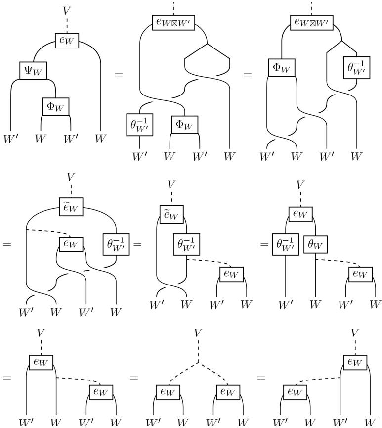
Proof of a key identity for showing rigidity, using graphical calculus from braided tensor category theory
